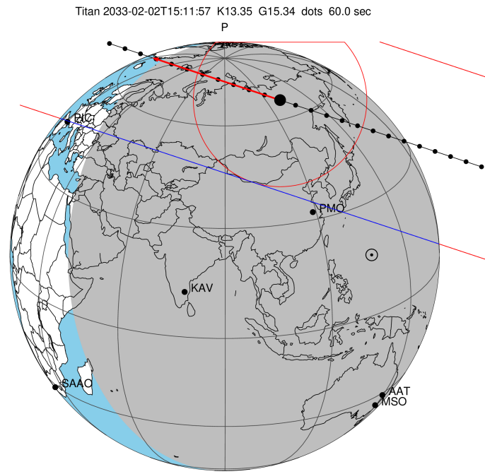
2033-02-02T15:11:57.3400 α: 06 01 56.2340 δ: +22 32 36.338 C/A 0.821" PA 18.36 deg v_sky - 8.09 km/s D 08.28 AU Credit: Styled after SORA/Lucky Star
