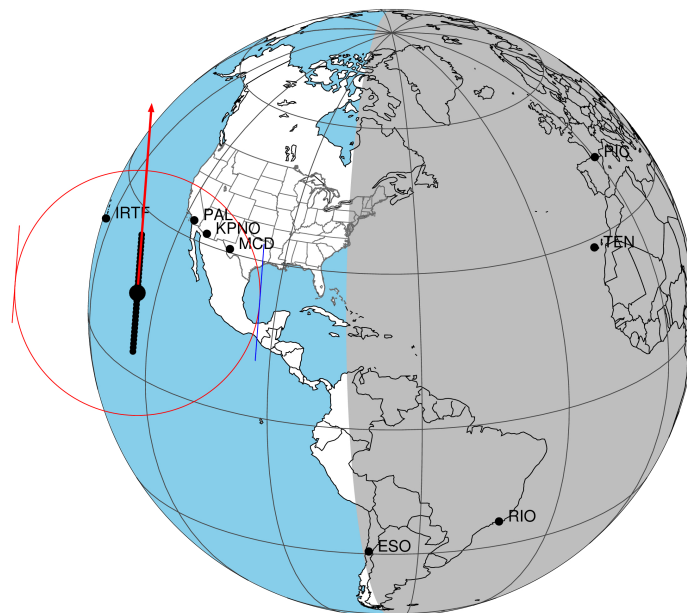
2033-03-11T23:04:40.7300 α: 05 59 25.4584 δ: +22 41 51.271 C/A 0.839" PA 274.33 deg v_sky + 1.37 km/s D 08.81 AU Credit: Styled after SORA/Lucky Star
