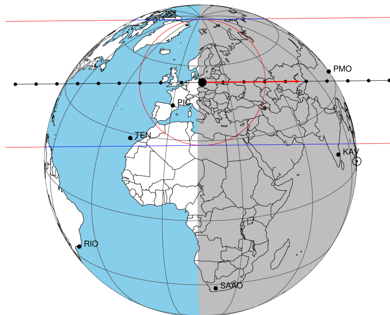
2033-03-19T17:14:58.7200 α: 06 00 07.7426 δ: +22 40 27.452 C/A 0.494" PA 359.40 deg v_sky +14.13 km/s D 08.95 AU Credit: Styled after SORA/Lucky Star
