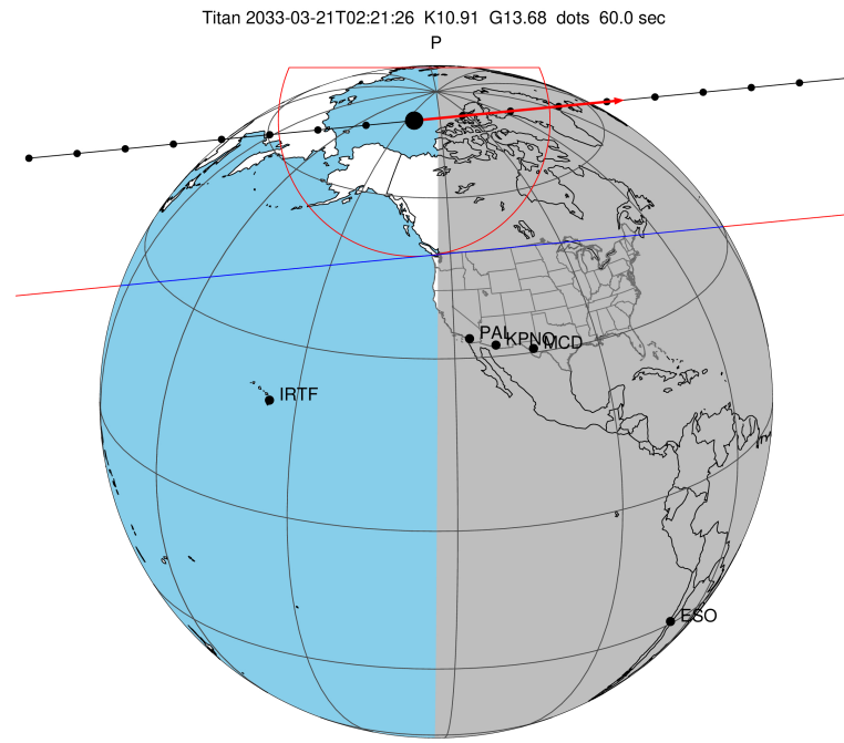
2033-03-21T02:21:26.9500 α: 06 00 27.3706 δ: +22 40 42.236 C/A 0.822" PA 354.40 deg v_sky +15.29 km/s D 08.97 AU Credit: Styled after SORA/Lucky Star
