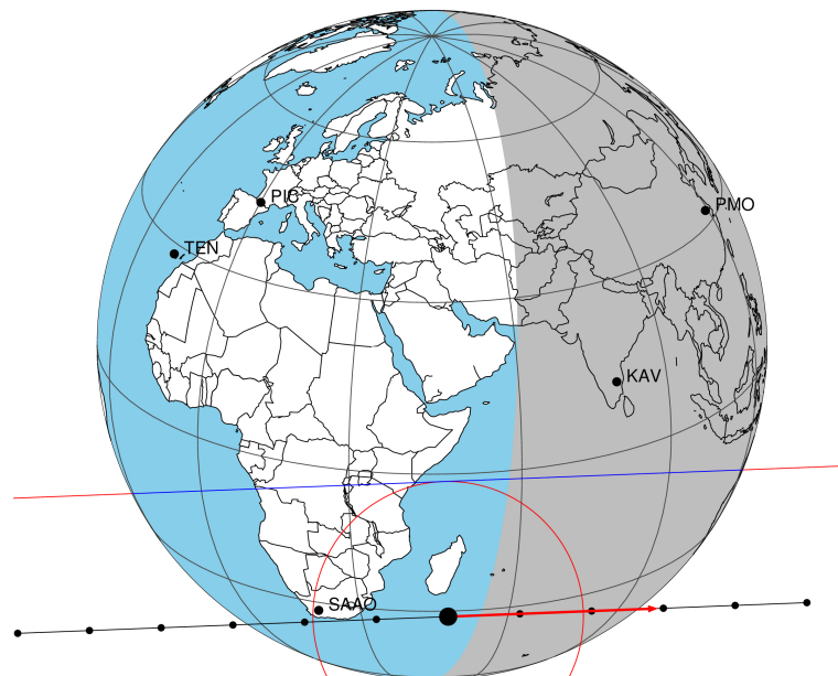
2033-04-05T14:11:13.5700 α: 06 03 43.1196 δ: +22 43 10.853 C/A 0.775" PA 177.76 deg v_sky +22.79 km/s D 09.23 AU Credit: Styled after SORA/Lucky Star
