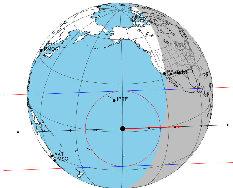
2033-04-22T02:15:24.6400 α: 06 09 03.3982 δ: +22 45 01.616 C/A 0.327" PA 178.02 deg v_sky +29.90 km/s D 09.48 AU Credit: Styled after SORA/Lucky Star
