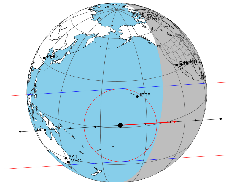
2033-04-23T03:23:16.8300 α: 06 09 31.7182 δ: +22 45 21.071 C/A 0.334" PA 176.36 deg v_sky +29.63 km/s D 09.49 AU Credit: Styled after SORA/Lucky Star
