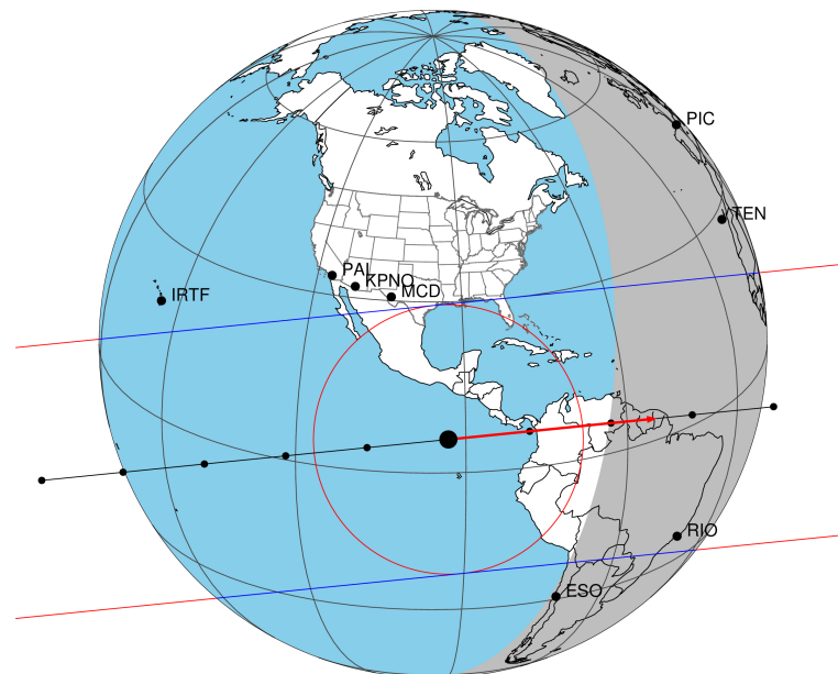
2033-04-25T22:18:22.9600 α: 06 10 42.3059 δ: +22 46 46.676 C/A 0.267" PA 174.26 deg v_sky +26.01 km/s D 09.53 AU Credit: Styled after SORA/Lucky Star
