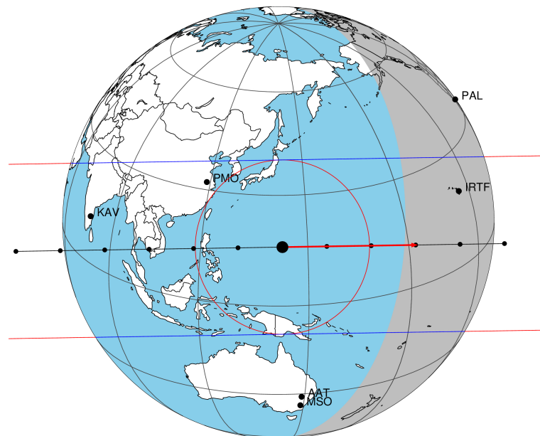
2033-04-29T06:16:21.5700 α: 06 11 52.9139 δ: +22 47 57.539 C/A 0.105" PA 179.11 deg v_sky +21.88 km/s D 09.57 AU Credit: Styled after SORA/Lucky Star
