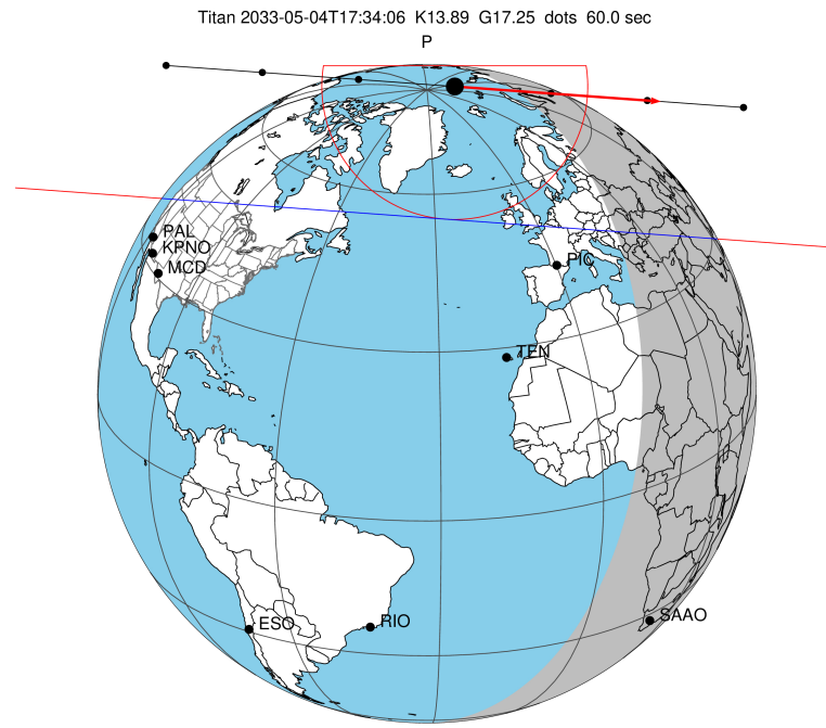
Titan 2033-05-04T17:34:06 K13.89 G17.25 dots 60.0 sec P 2033-05-04T17:34:06.1900 cc: 06 13 55.81233 s: +22 46 00.650 C/A 0.854" PA 4.17 deg v_sky +31.15 km/s D 09.65 AU Credit: Styled after SORA/Lucky Star
