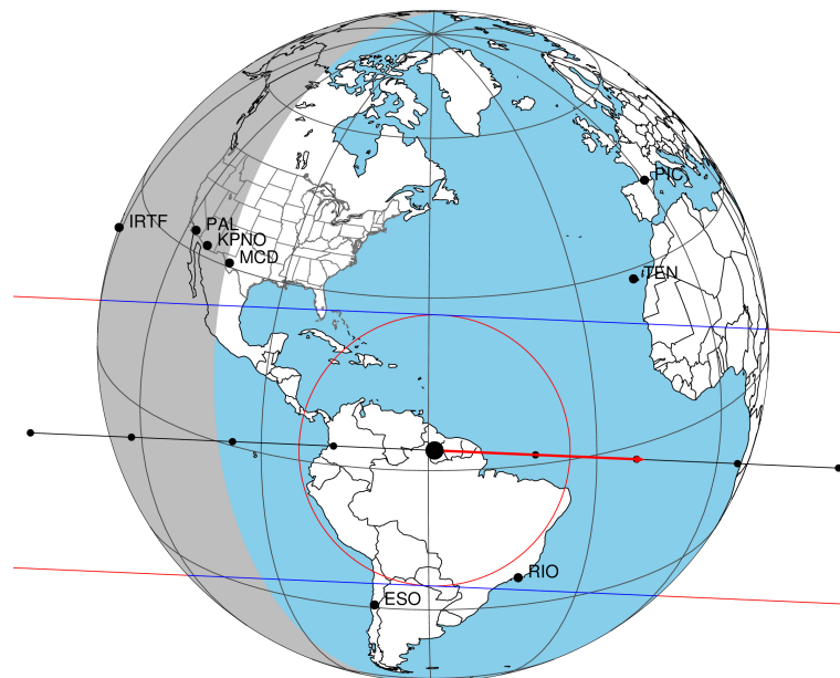
2033-08-30T12:37:58.8600 α: 07 15 19.5194 δ: +21 51 22.687 C/A 0.283" PA 182.52 deg v_sky +32.01 km/s D 09.65 AU Credit: Styled after SORA/Lucky Star
