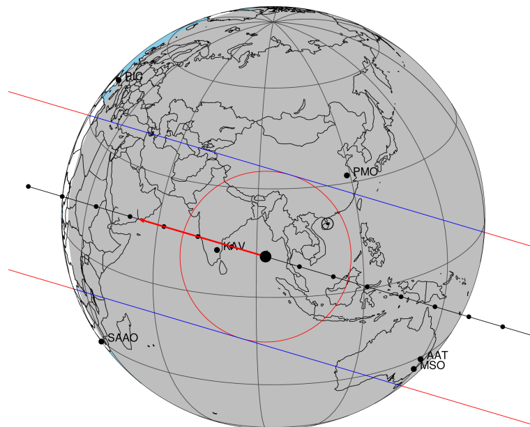
2034-01-21T16:49:40.0200 α: 07 10 38.5281 δ: +22 10 17.640 C/A 0.202" PA 196.50 deg v_sky -17.73 km/s D 08.08 AU Credit: Styled after SORA/Lucky Star
