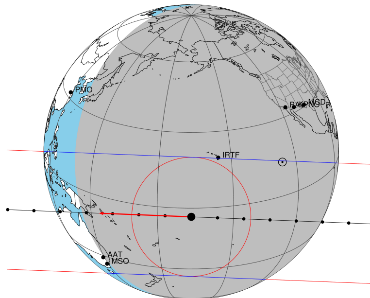
2034-02-12T08:42:48.5700 α: 07 04 01.2666 δ: +22 24 31.038 C/A 0.468" PA 182.25 deg v_sky -18.92 km/s D 08.23 AU Credit: Styled after SORA/Lucky Star
