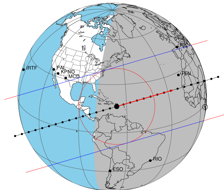
2034-03-25T23:25:23.4100 α: 07 00 49.9525 δ: +22 33 04.427 C/A 0.110" PA 163.71 deg v_sky + 7.93 km/s D 08.83 AU Credit: Styled after SORA/Lucky Star
