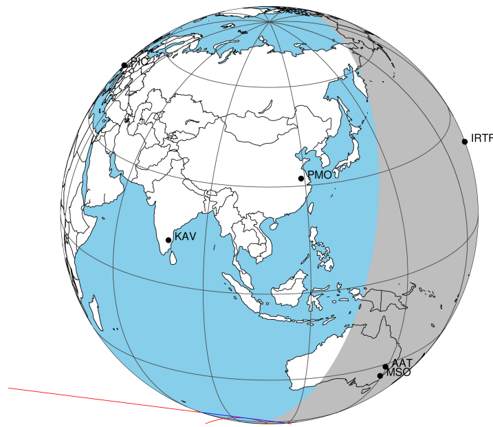
2034-05-08T08:53:42.2000 α: 07 10 46.1777 δ: +22 20 54.715 C/A 1.276" PA 187.21 deg v_sky +29.28 km/s D 09.53 AU Credit: Styled after SORA/Lucky Star
