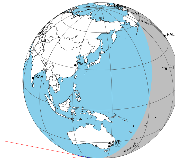
2034-05-19T06:03:18.3700 α: 07 15 11.6825 δ: +22 16 28.853 C/A 1.273" PA 191.06 deg v_sky +23.97 km/s D 09.66 AU Credit: Styled after SORA/Lucky Star
