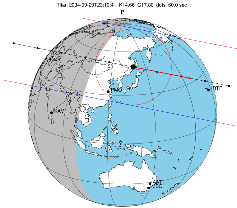
Titan 2034-09-29T23:10:41 K14.66 G17.80 dots 60.0 sec P 2034-09-29T23:10:41.3800 α: 08 20 42.7077 δ: +19 38 40.462 C/A 0.461" PA 11.22 deg v_sky +27.45 km/s D 09.47 AU Credit: Styled after SORA/Lucky Star
