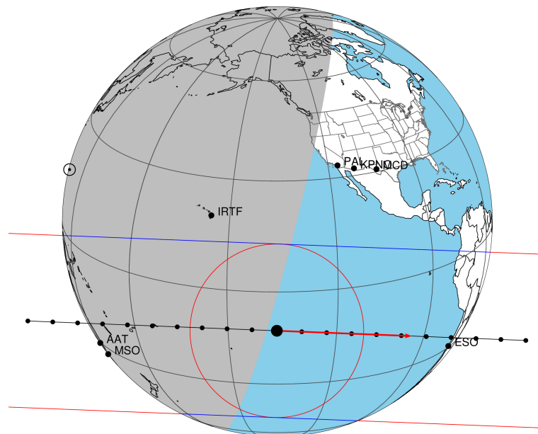
2034-11-02T14:48:15.5700 α: 08 28 26.1903 δ: +19 16 42.833 C/A 0.500" PA 182.24 deg v_sky +12.32 km/s D 08.93 AU Credit: Styled after SORA/Lucky Star
