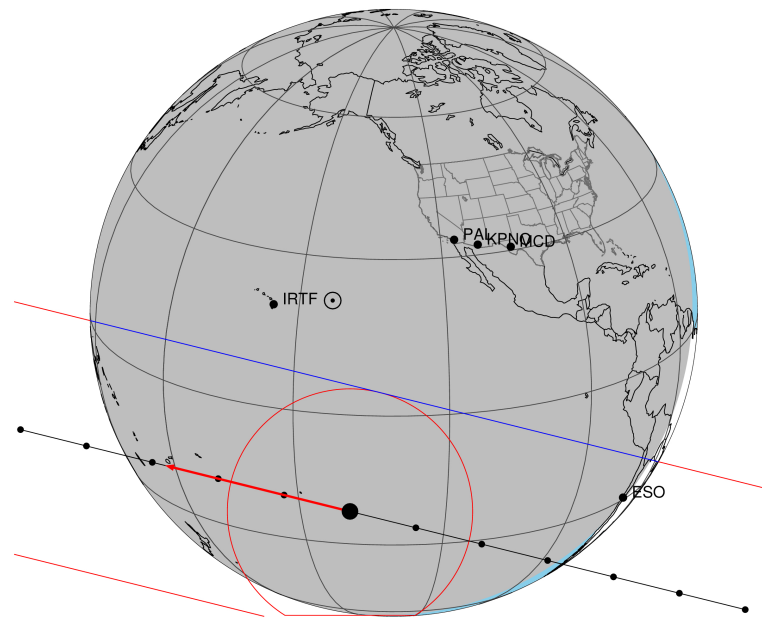
2035-01-11T09:40:13.4300 α: 08 18 46.0903 δ: +20 01 09.841 C/A 0.727" PA 193.97 deg v_sky -23.76 km/s D 08.10 AU Credit: Styled after SORA/Lucky Star
