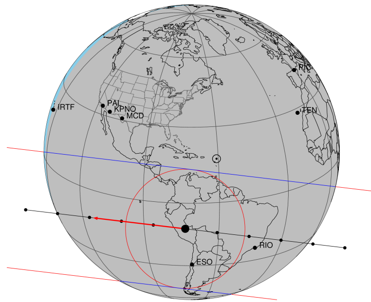
2035-01-31T04:16:09.4100 α: 08 11 45.1442 δ: +20 24 04.572 C/A 0.566" PA 186.79 deg v_sky -23.10 km/s D 08.10 AU Credit: Styled after SORA/Lucky Star
