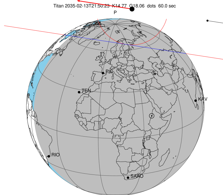
2035-02-13T21:50:23.3700 α: 08 07 36.0951 δ: +20 39 20.580 C/A 1.209" PA 8.75 deg v_sky -22.82 km/s D 08.17 AU Credit: Styled after SORA/Lucky Star
