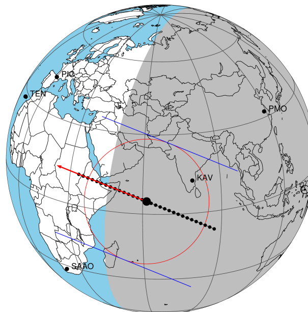
2035-03-31T15:00:19.1400 cc: 08 00 40.0804 d: +21 02 56.426 C/A 0.290" PA 201.96 deg v_sky - 3.35 km/s D 08.73 AU Credit: Styled after SORA/Lucky Star
