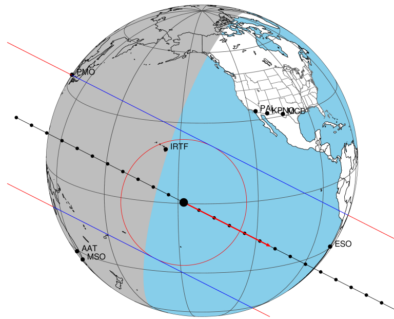
2035-10-28T16:20:48.4600 α: 09 21 45.5325 δ: +16 14 24.455 C/A 0.276" PA 206.87 deg v_sky +11.64 km/s D 09.29 AU Credit: Styled after SORA/Lucky Star
