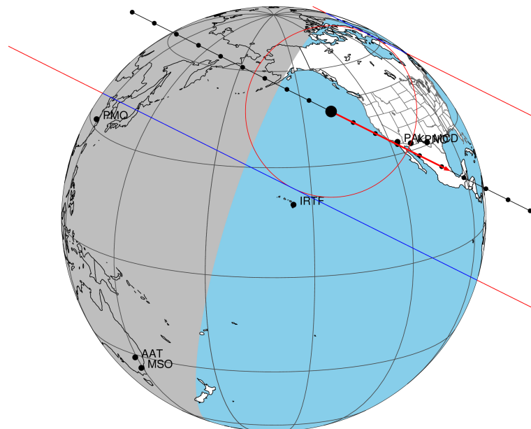
2035-10-29T17:36:52.2500 α: 09 21 55.4960 δ: +16 13 10.627 C/A 0.543" PA 26.50 deg v_sky +12.37 km/s D 09.28 AU Credit: Styled after SORA/Lucky Star
