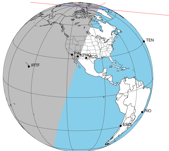
2035-11-07T13:44:50.6800 cc: 09 24 00.2004 &: +16 06 06.312 C/A 1.288" PA 5.44 deg v_sky +14.02 km/s D 09.14 AU Credit: Styled after SORA/Lucky Star
