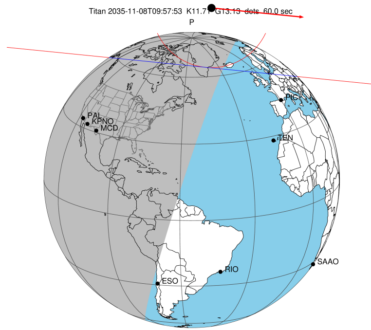
2035-11-08T09:57:53.7000 cc: 09 24 10.0848 & +16 05 52.709 C/A 1.129" PA 5.75 deg v_sky +12.00 km/s D 09.13 AU Credit: Styled after SORA/Lucky Star
