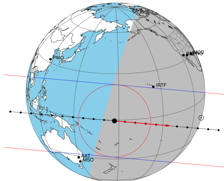
2036-04-29T06:38:59.3900 \alpha : 08 59 25.9067 \delta : +18 10 47.675 C/A 0.309" PA 185.08 deg v_sky +12.41 km/s D 09.06 AU Credit: Styled after SORA/Lucky Star
