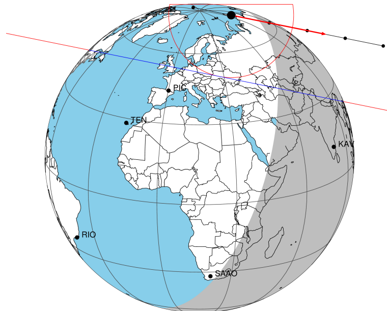
2036-05-31T15:25:43.3800 α: 09 06 38.7036 δ: +17 39 37.962 C/A 0.870" PA 11.45 deg v_sky +26.65 km/s D 09.58 AU Credit: Styled after SORA/Lucky Star
