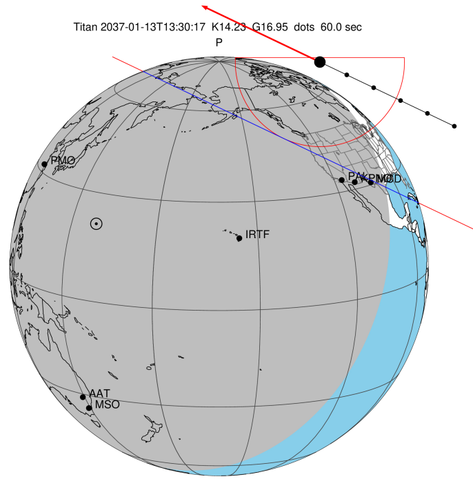
2037-01-13T13:30:17.5100 cc: 10 16 27.8748 d: +12 22 51.158 C/A 1.134" PA 25.50 deg v_sky -15.13 km/s D 08.43 AU Credit: Styled after SORA/Lucky Star
