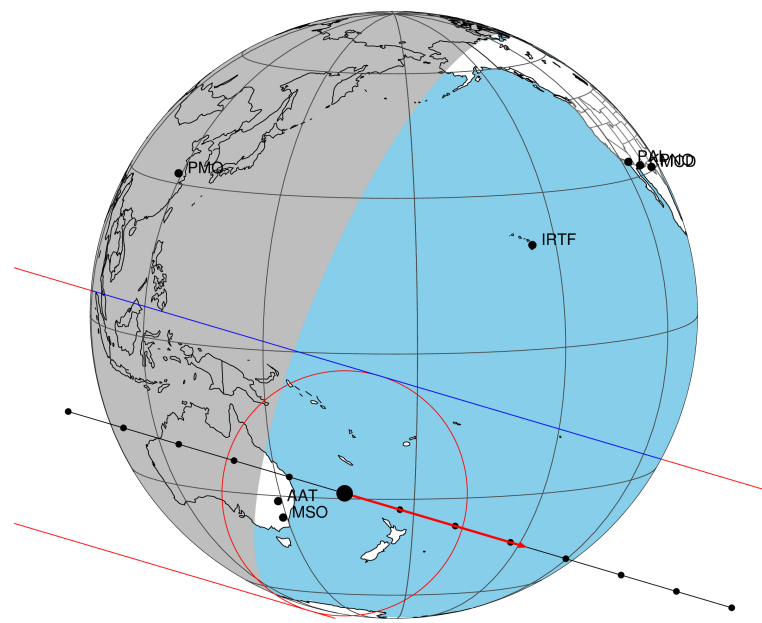
2037-11-21T19:21:12.4700 \alpha : 11 05 55.7841 \delta : +07 38 09.892 C/A 0.563" PA 196.48 deg v_sky +20.18 km/s D 09.53 AU Credit: Styled after SORA/Lucky Star
