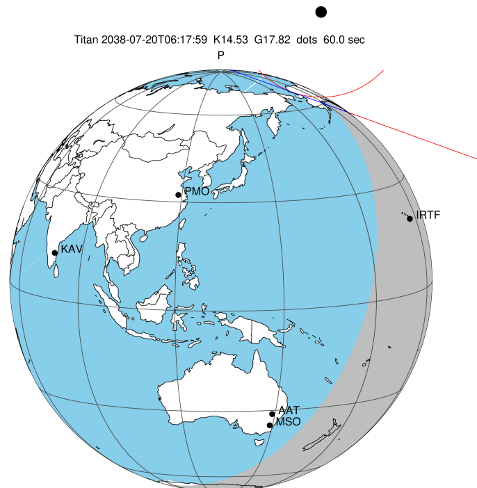
2038-07-20T06:17:59.9800 α: 10 59 02.5603 δ: +08 30 24.615 C/A 1.186" PA 19.90 deg v_sky +34.77 km/s D 10.07 AU Credit: Styled after SORA/Lucky Star
