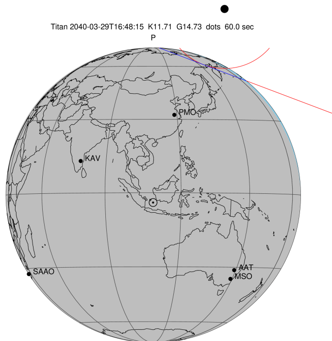
2040-03-29T16:48:15.9900 α: 12 33 34.8022 δ: -00 44 05.932 C/A 1.388" PA 20.72 deg v_sky -23.60 km/s D 08.57 AU Credit: Styled after SORA/Lucky Star
