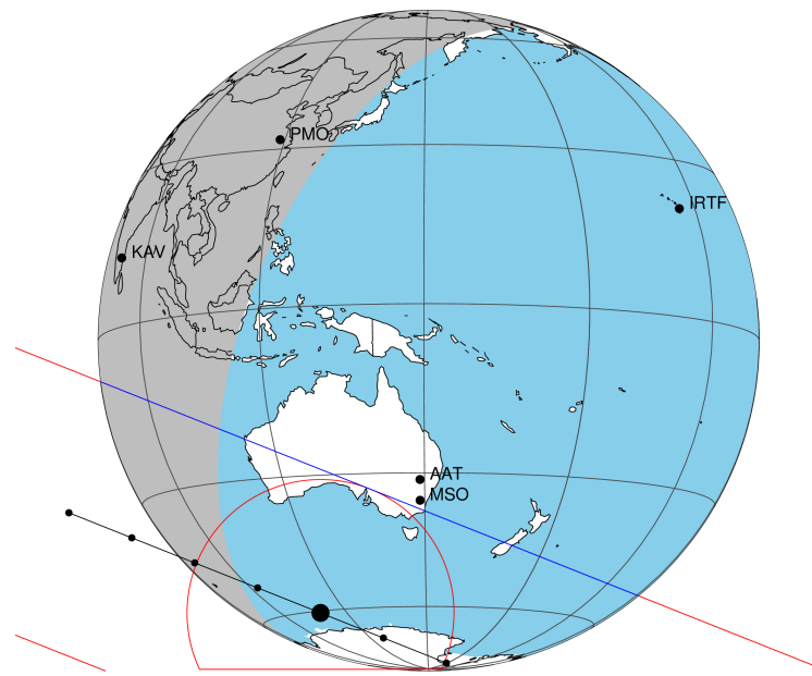
2040-12-09T22:04:25.5400 α: 13 22 42.8804 δ: -06 11 52.616 C/A 0.768" PA 201.72 deg v_sky +21.77 km/s D 10.15 AU Credit: Styled after SORA/Lucky Star
