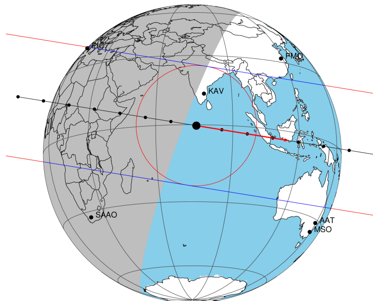
2042-01-19T01:26:46.4400 α: 14 15 51.1399 δ: -11 00 10.010 C/A 0.169" PA 9.19 deg v_sky +18.40 km/s D 09.84 AU Credit: Styled after SORA/Lucky Star
