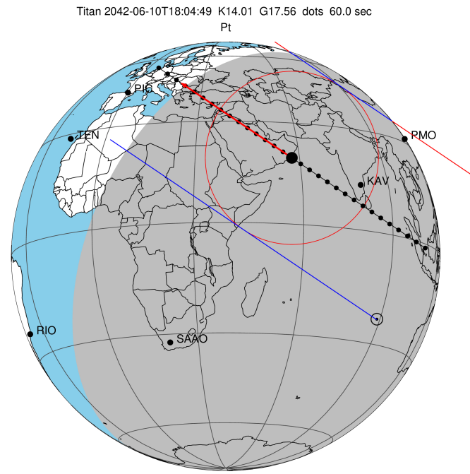
2042-06-10T18:04:49.2400 α: 13 54 09.1800 δ: -08 53 34.285 C/A 0.534" PA 34.05 deg v_sky - 5.32 km/s D 09.12 AU Credit: Styled after SORA/Lucky Star
