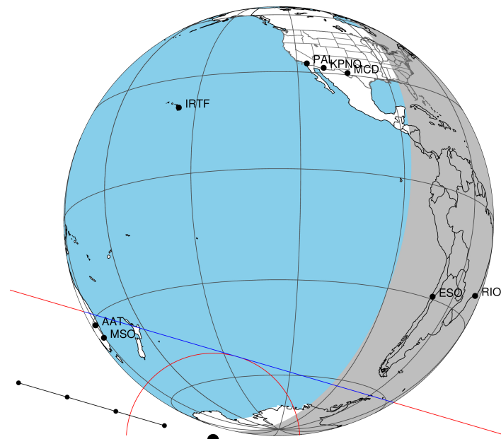
2043-09-12T23:46:35.6400 α: 14 48 16.1002 δ: -13 58 55.307 C/A 0.895" PA 196.36 deg v_sky +25.07 km/s D 10.45 AU Credit: Styled after SORA/Lucky Star
