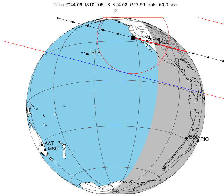
2044-09-13T01:06:18.3100 cc: 15 31 18.1172 s: -17 05 36.766 C/A 0.676" PA 14.65 deg v_sky +18.50 km/s D 10.35 AU Credit: Styled after SORA/Lucky Star
