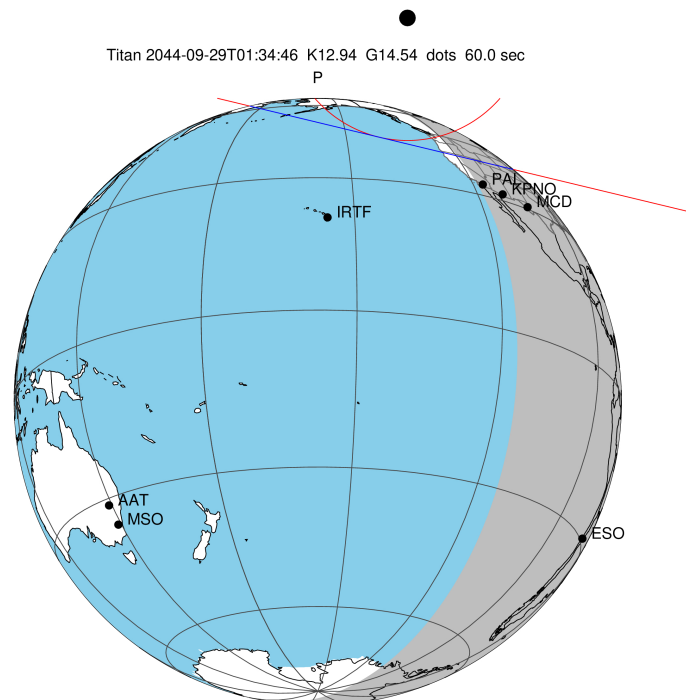
2044-09-29T01:34:46.7900 cc: 15 36 31.7670 d: -17 27 02.825 C/A 1.080" PA 13.53 deg v_sky +24.82 km/s D 10.58 AU Credit: Styled after SORA/Lucky Star
