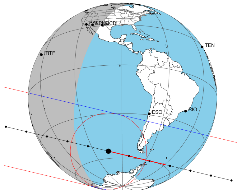
2045-01-29T13:55:19.5600 α: 16 31 02.6616 δ: -20 02 18.274 C/A 0.497" PA 193.41 deg v_sky +23.72 km/s D 10.43 AU Credit: Styled after SORA/Lucky Star
