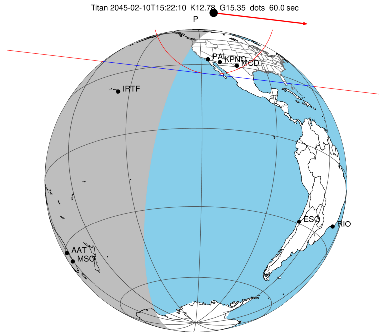
2045-02-10T15:22:10.0500 α: 16 34 25.4928 δ: -20 06 56.539 C/A 0.956" PA 6.73 deg v_sky +24.42 km/s D 10.26 AU Credit: Styled after SORA/Lucky Star
