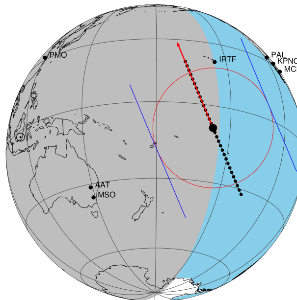
2045-03-26T16:26:07.2600 α: 16 39 09.3999 δ: -20 11 37.507 C/A 0.391" PA 67.33 deg v_sky - 3.44 km/s D 09.54 AU Credit: Styled after SORA/Lucky Star
