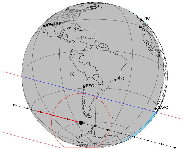
2045-05-12T05:16:33.7800 cc: 16 30 41.2989 s: -19 51 07.885 C/A 0.662" PA 194.91 deg v_sky -20.24 km/s D 09.03 AU Credit: Styled after SORA/Lucky Star
