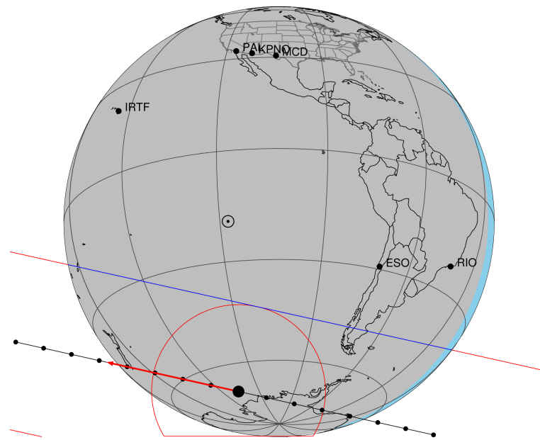
2045-05-16T07:46:49.0900 cc: 16 29 39.5230 r: -19 47 05.220 C/A 0.791" PA 192.54 deg v_sky -14.09 km/s D 09.02 AU Credit: Styled after SORA/Lucky Star
