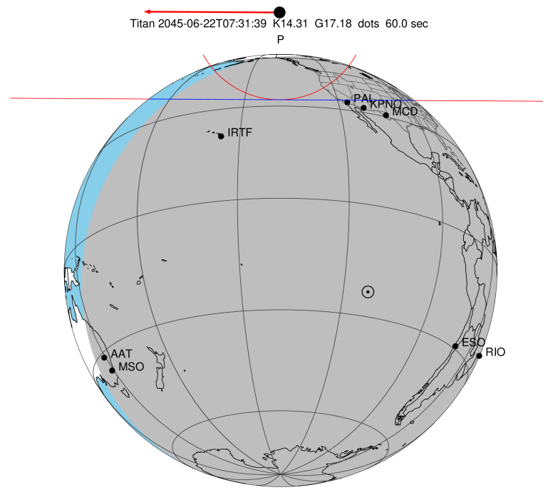
2045-06-22T07:31:39.7200 α: 16 18 45.4224 δ: -19 26 13.103 C/A 1.158" PA 0.33 deg v_sky -19.25 km/s D 09.07 AU Credit: Styled after SORA/Lucky Star
