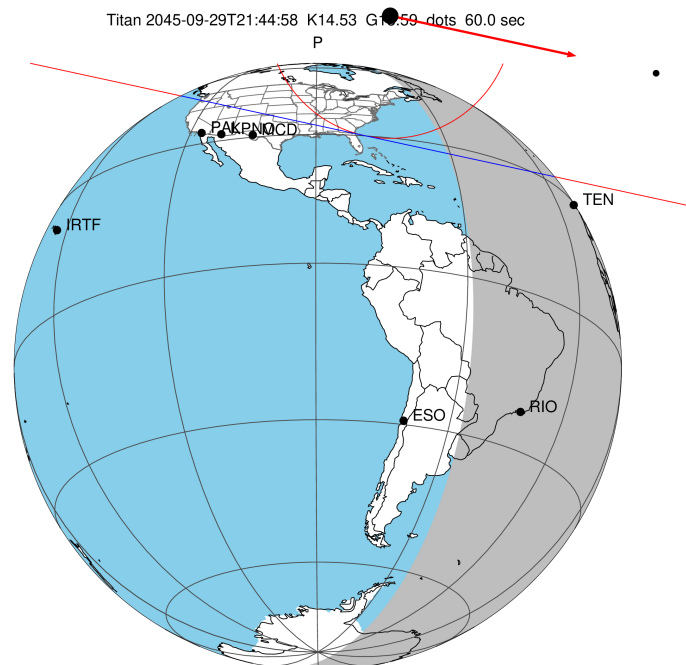
2045-09-29T21:44:58.2300 cc: 16 20 11.1171 d: -19 52 01.589 C/A 0.992" PA 12.21 deg v_sky +19.04 km/s D 10.47 AU Credit: Styled after SORA/Lucky Star
