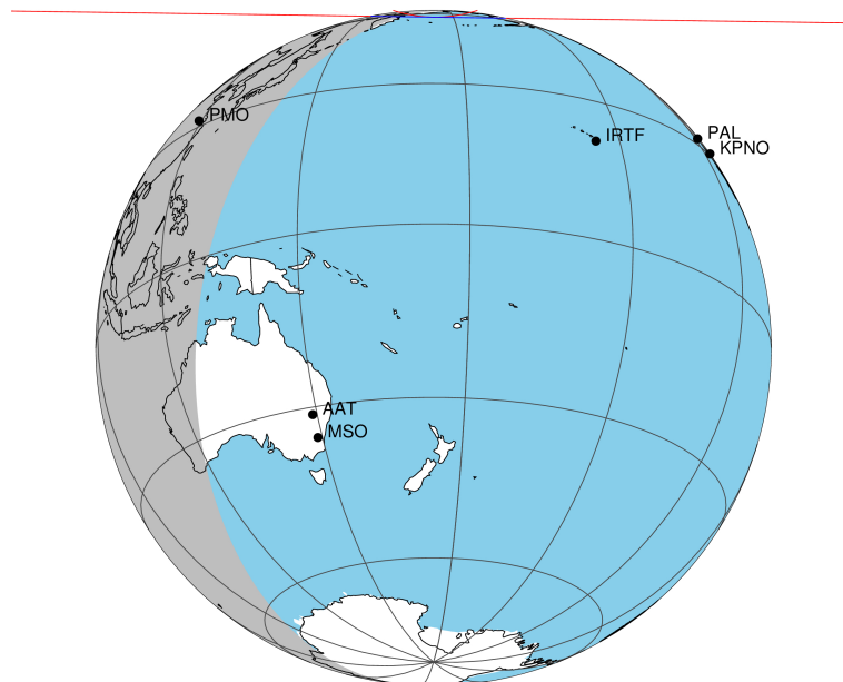
2046-01-24T21:23:07.8300 α: 17 13 08.5831 δ: -21 32 20.570 C/A 1.137" PA 0.82 deg v_sky +33.52 km/s D 10.70 AU Credit: Styled after SORA/Lucky Star
