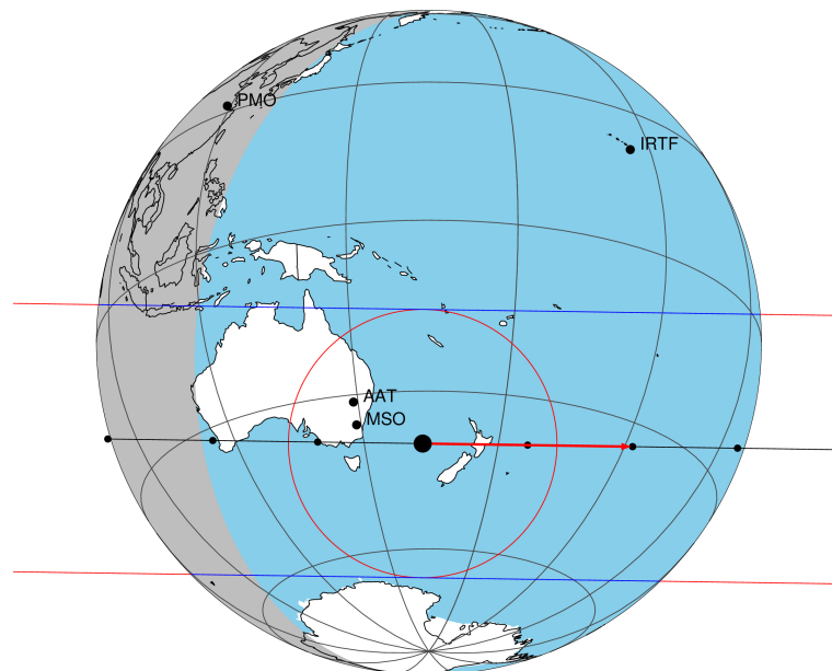
2046-01-24T22:00:23.4300 α: 17 13 09.2771 δ: -21 32 19.322 C/A 0.250" PA 180.86 deg v_sky +33.55 km/s D 10.70 AU Credit: Styled after SORA/Lucky Star
