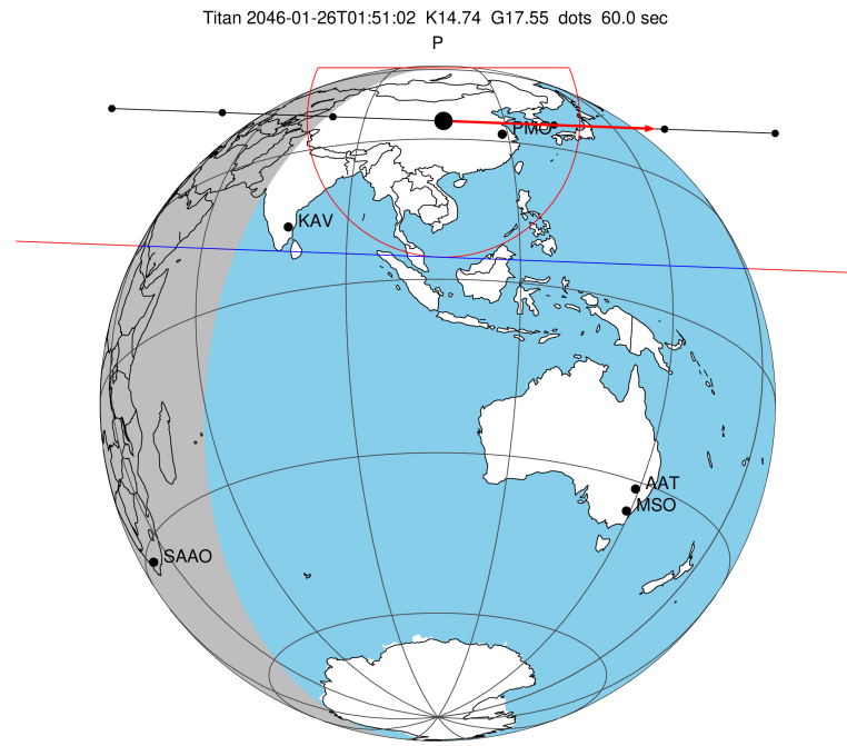
2046-01-26T01:51:02.4500 α: 17 13 41.0019 δ: -21 32 31.569 C/A 0.688" PA 2.15 deg v_sky +34.83 km/s D 10.68 AU Credit: Styled after SORA/Lucky Star
