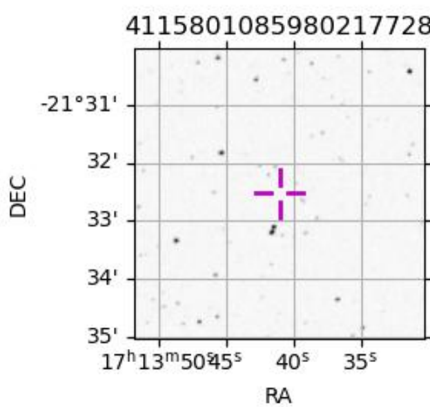
2046-01-26T01:51:02.4500 α: 17 13 41.0019 δ: -21 32 31.569 C/A 0.688" PA 2.15 deg v_sky +34.83 km/s D 10.68 AU Credit: Styled after SORA/Lucky Star
