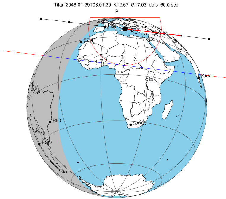
2046-01-29T08:01:29.5200 α: 17 15 11.3435 δ: -21 34 10.197 C/A 0.726" PA 6.89 deg v_sky +33.27 km/s D 10.64 AU Credit: Styled after SORA/Lucky Star
