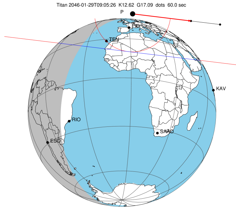
2046-01-29T09:05:26.7300 α: 17 15 12.5177 δ: -21 34 12.331 C/A 0.871" PA 6.95 deg v_sky +33.19 km/s D 10.64 AU Credit: Styled after SORA/Lucky Star
